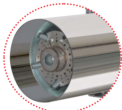
Example of a RS/M MZ burner combustion head
