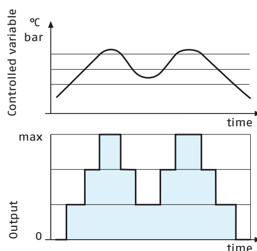
Three stage operation
