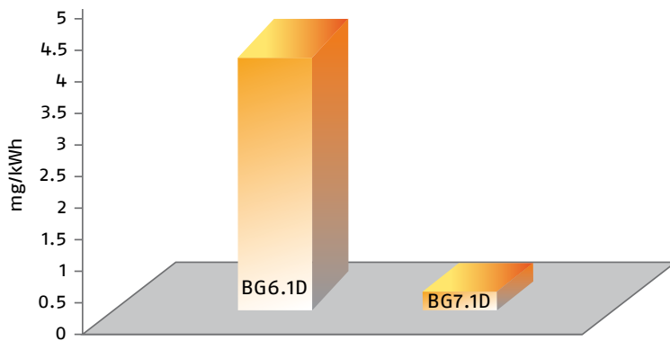
CO EMISSIONS
