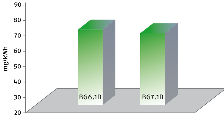
NO2 EMISSIONS
